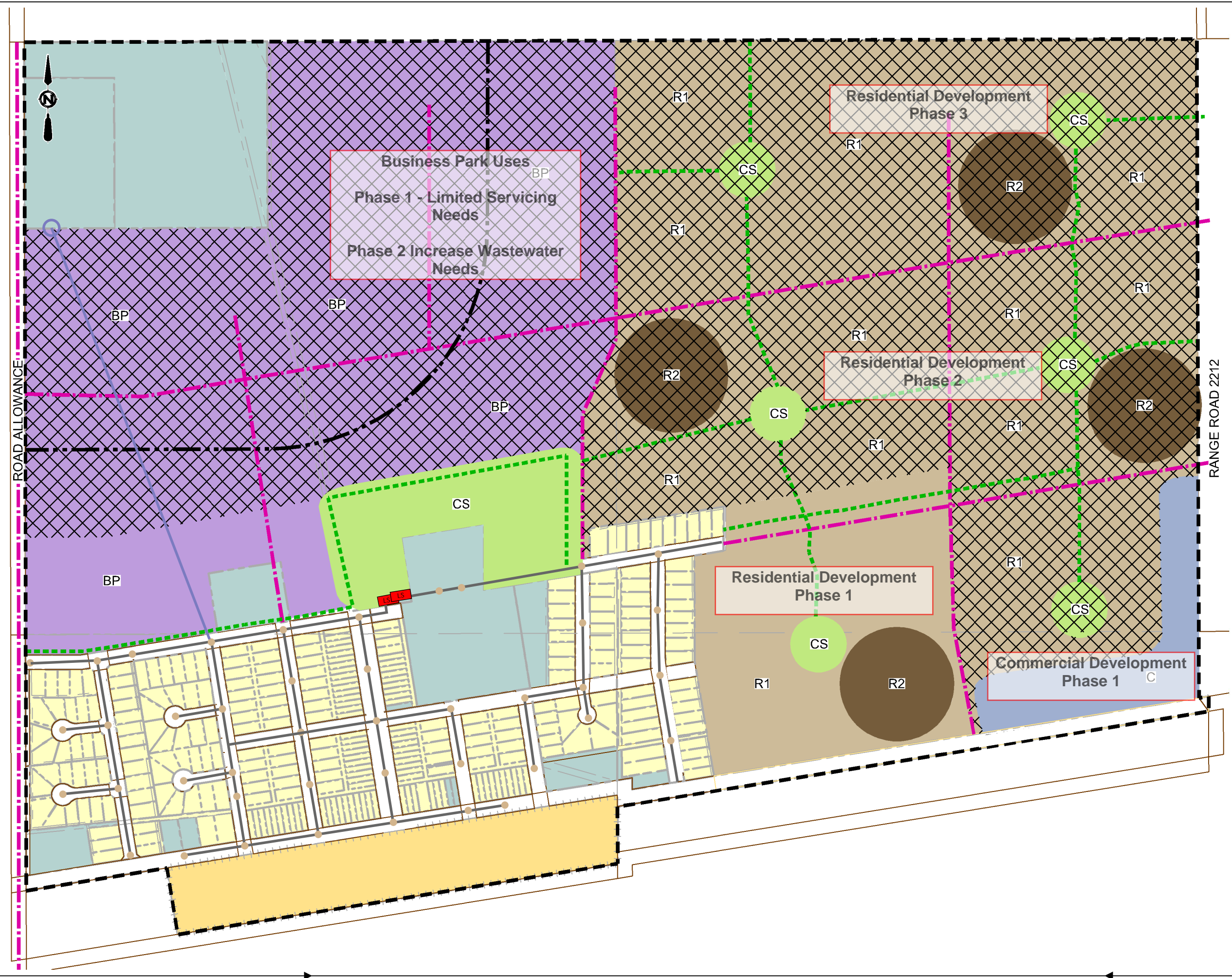
APPENDIX "D2" Future Growth Sewage Servicing Map TOWN OF GRAND COULEE
